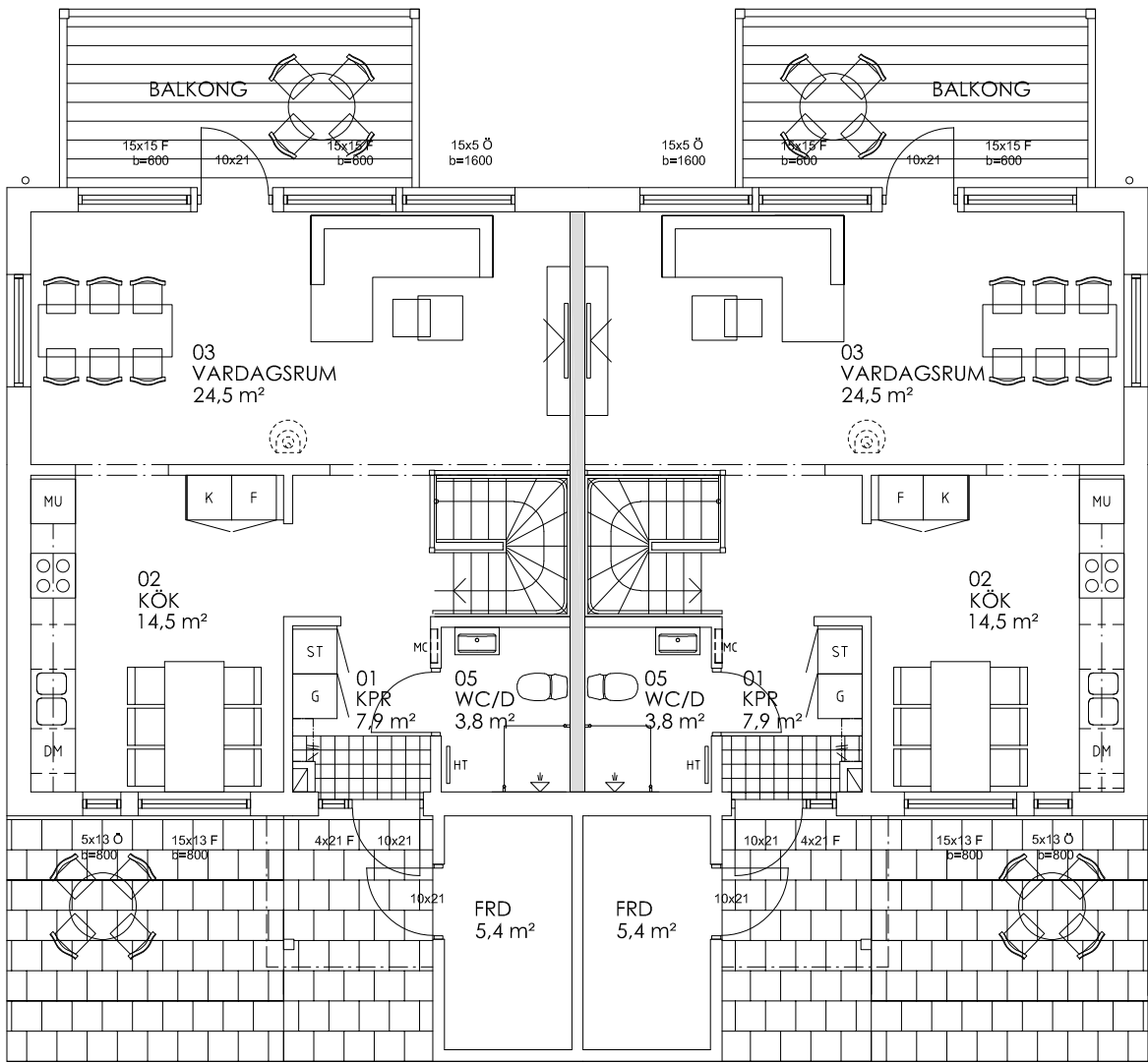
PLAN 1
