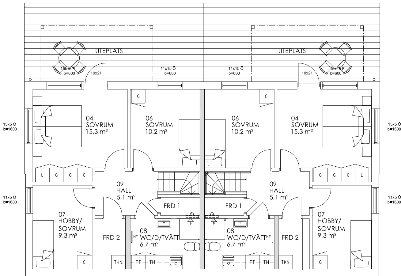
PLAN 0
